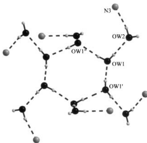
Figure 2. A simplified view of the dodecameric water cluster. Distances [Å]: Ow1...Ow2 2.827(6), Ow1...Ow1' 2.801(6); angles [°]: Ow2...H-Ow1 172.26(2), Ow1...H-Ow1' 173.65(2), Ow1'...Ow1...Ow1'' 119.58(1), Ow2...Ow1...Ow1' 109.36(2), Ow2...Ow1...Ow1'' 104.38(2).
